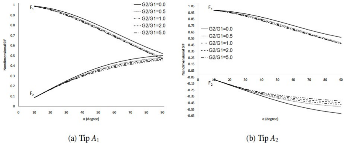
Figure 6: Nondimensional SIF versus \alpha subjected to Mix Mode stress at crack tips
