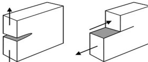
Figure 1: Three types of mode stresses in fracture mechanics
