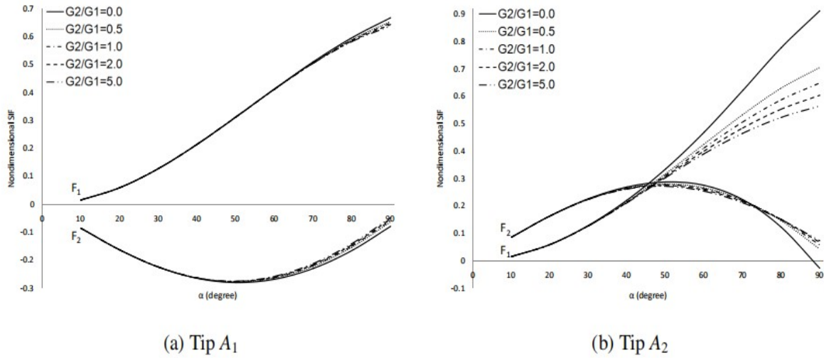
Figure 3: Nondimensional SIF versus \alpha subjected to Mode I stress at crack tips
