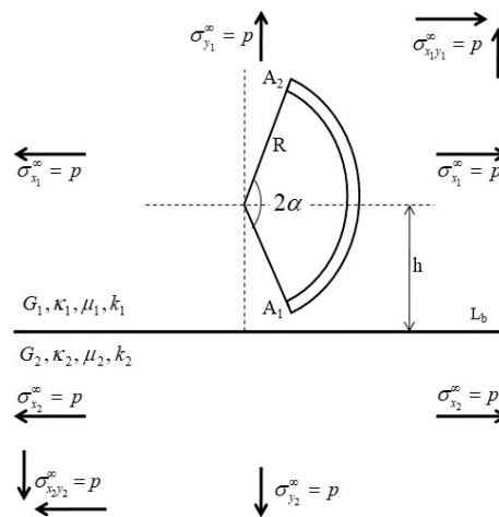
Figure 2: A thermally insulated curve crack in the upper side of bonded two half planes
