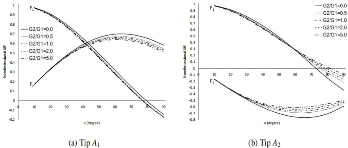
Figure 4: Nondimensional SIF versus \alpha subjected to Mode II stress at crack tips
