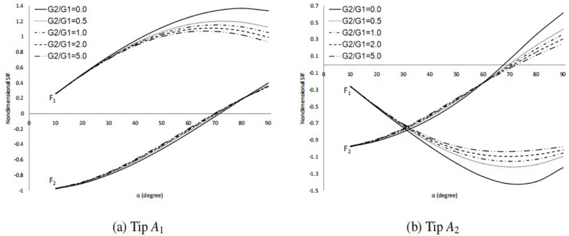
Figure 5: Nondimensional SIF versus \alpha subjected to Mode III stress at crack tips
